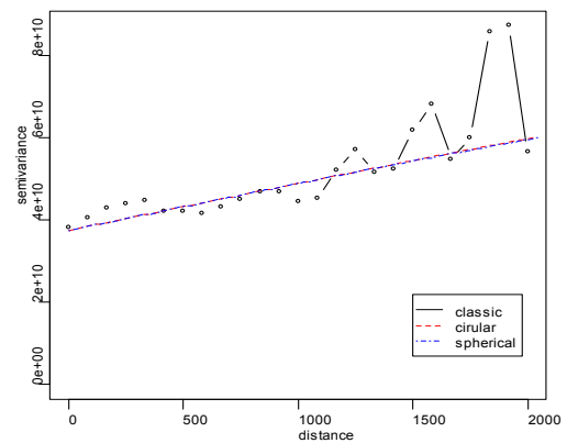
Figure 2 Plot of variogram and fitted Models for the the Gini Coefficient of expenses
